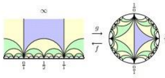
Figure 3. The tessellation of the upper half plane by ideal triangles according to the Farey
