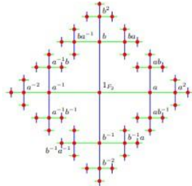
Figure 7. A Cayley graph for F_2
