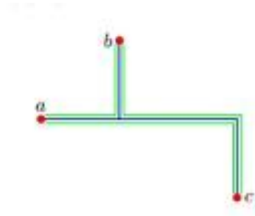
Figure 10. One of the most common geodesic triangles seen in trees
