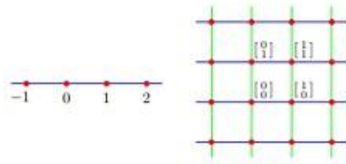
Figure 5. Cayley graphs for \mathbb{Z} and \mathbb{Z}^2
