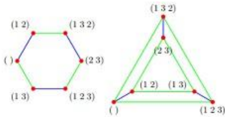
Figure 6. Cayley graphs for \text{Sym}(3)
